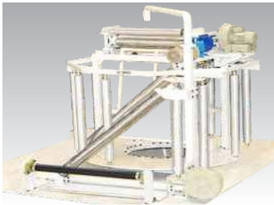
Vertical Haul-off
